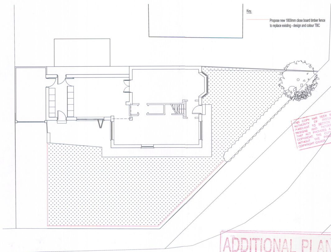
● Proposed Site Plan Scale: 1:100 @ A3
